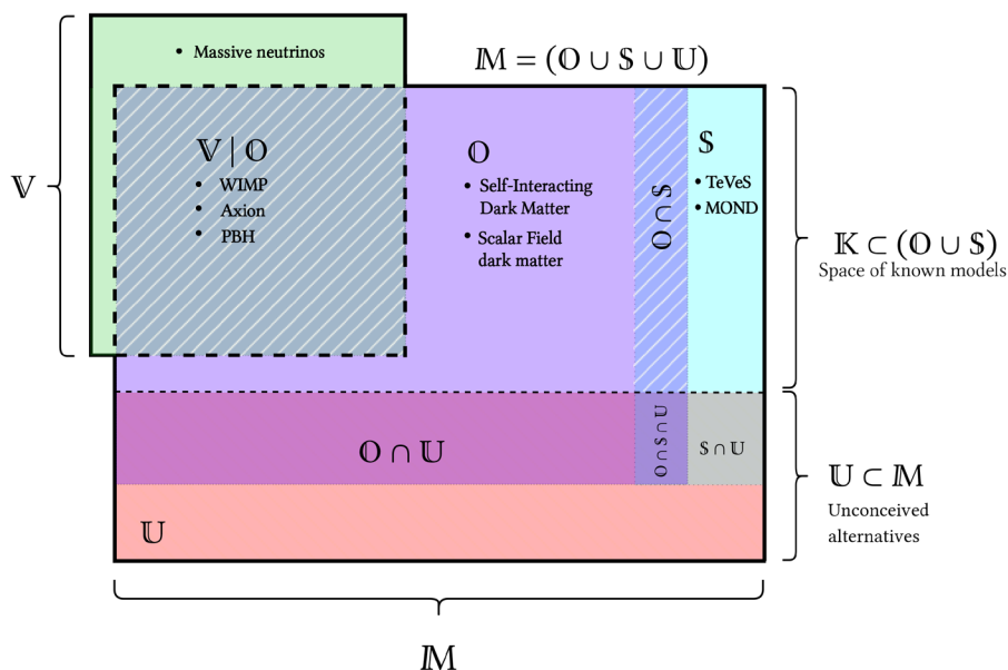
Fig. 1 Model-space. Y axis is split between known and unknown models, the X axis is split between object and structure based models. The shaded area is the Vaynberg constraint V , and PBH is the abbreviation of primordial black holes
